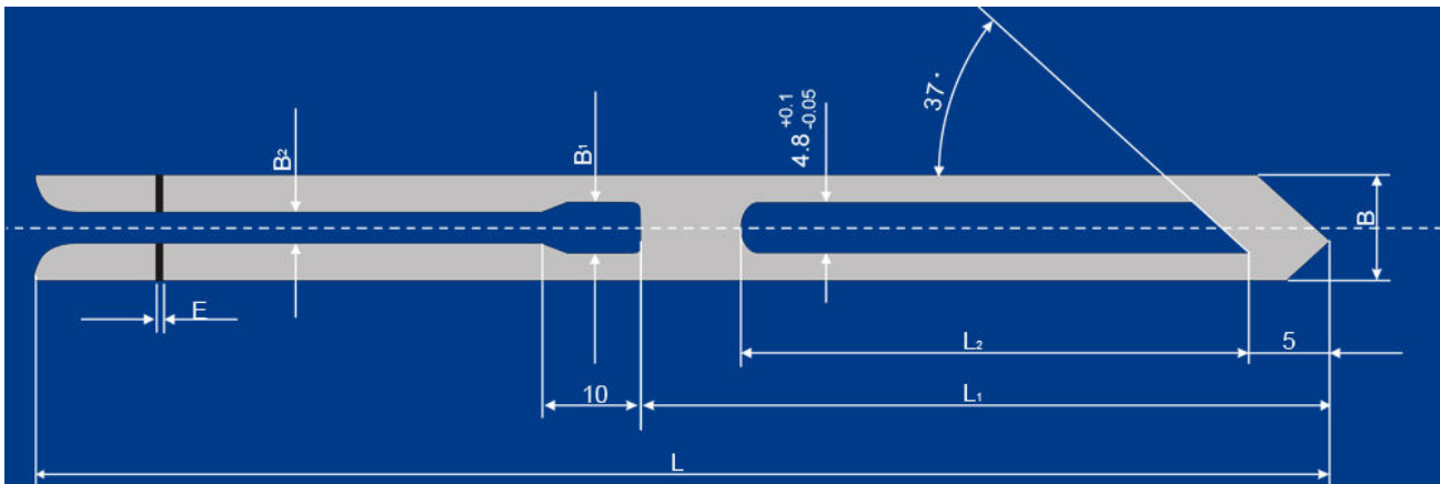
Open, U type thread eye
