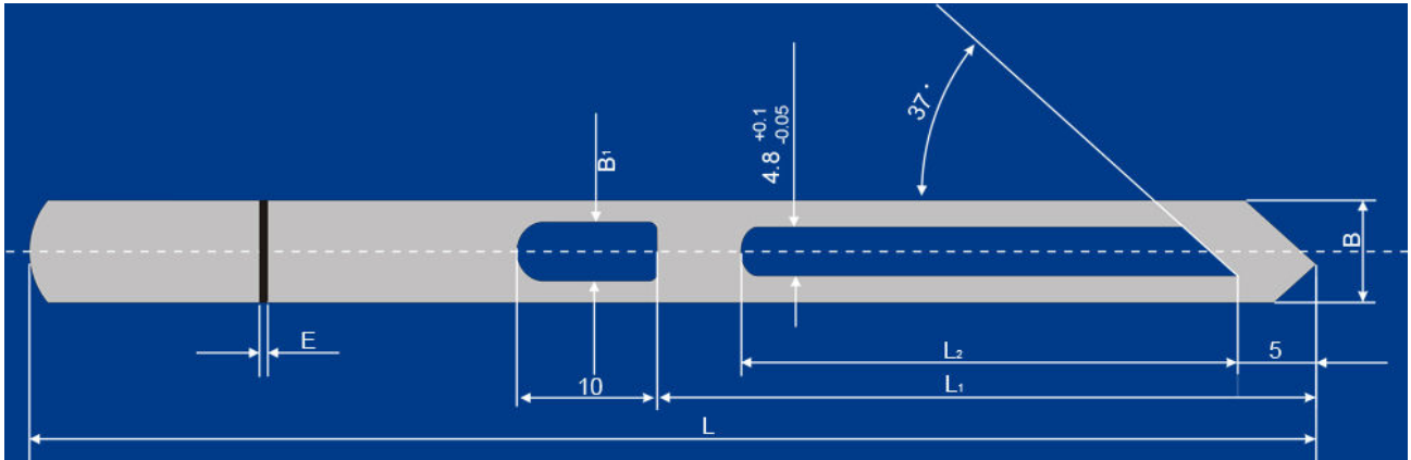
Closed, U type thread eye
